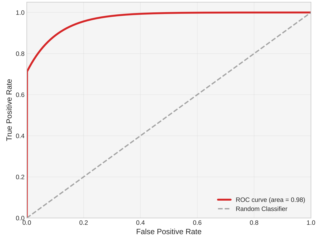
SVM: ROC Curve
